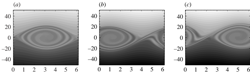
FIGURE 3. Plots of the vorticity inside the critical layer using a grey-scale representation for the cases \mathcal{D}_2=0, +0.3, -0.3 (a–c respectively) at T=4.5, 5.0 and 5 .
