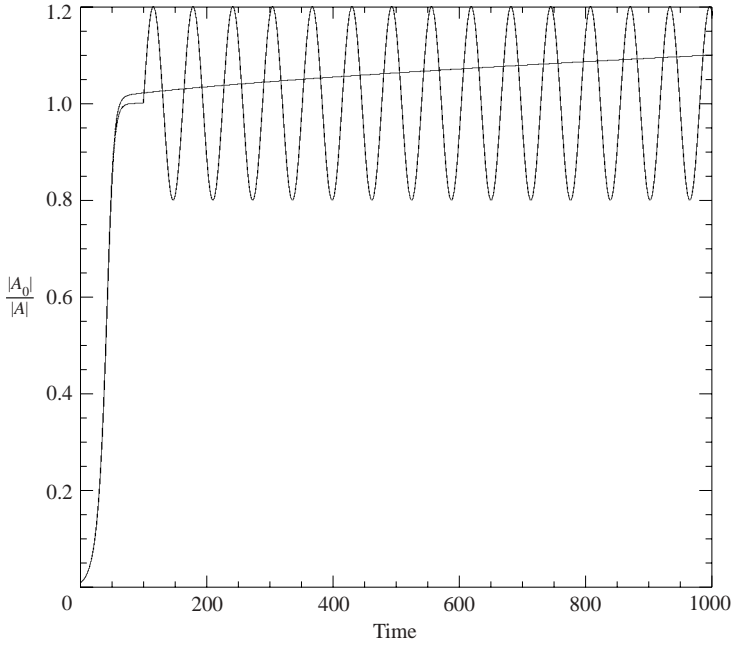
FIGURE 7. The two classes of model for the amplitude R used in calculating the particle dispersion: the first class, corresponding to inviscid critical layers, shows initial exponential growth followed by saturation to R \sim 1 and oscillatory behaviour; the second class, corresponding to the viscous case, follows the exponential phase with algebraic growth. We show only the oscillatory case with period 65; the shorter-period (6) case looks identical but for the period of the oscillation, but cannot be easily displayed on the same time plot for reasons of graphical clarity.
