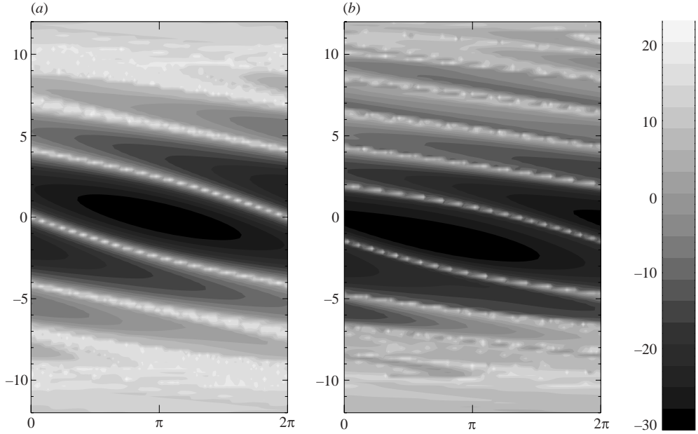
FIGURE 4. (a) \langle \lambda_0 \rangle for the critical layer without coupling to the gravity wave ( \mathcal{D}_2 = 0 ). (b) \langle \lambda_0 \rangle for the critical layer coupled to the gravity wave ( \mathcal{D}_2 = 0.2 ). Bright regions indicate possible positive Lyapunov exponent.
