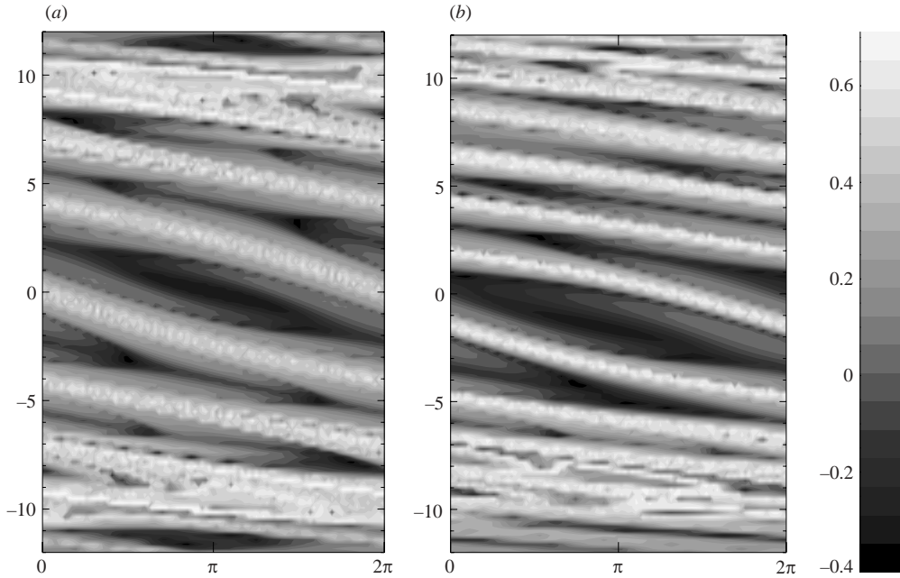
FIGURE 5. (a) Finite-time Lyapunov exponent the uncoupled case \mathcal{D}_2=0 . (b) Finite-time Lyapunov exponent for the case \mathcal{D}_2=0.2 . Bright regions indicate positive Lyapunov exponent.
