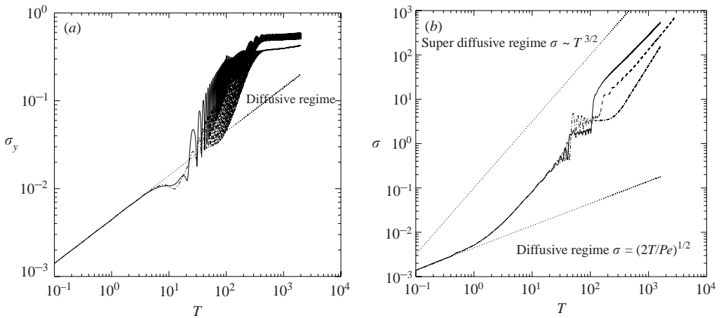
FIGURE 8. Results of our particle dispersion calculations, for the three amplitude models shown in the previous figure; in each panel, the solid line corresponds to the oscillatory case with period 6; the long dashed line to the oscillatory case with period 65; and the dash-dotted line to the viscous case, with ultimately algebraic amplitude growth. We show the particle dispersion \sigma in (a) the transverse direction and (b) the longitudinal direction.
