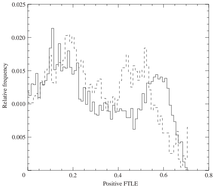
FIGURE 6. Probability distribution of the positive finite-time Lyapunov exponent. Dashed line corresponds to figure 5(a), and solid line corresponds to figure 5(b).
