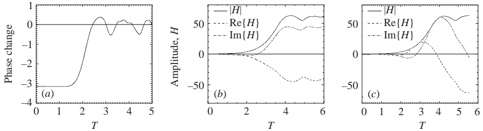
FIGURE 2. The evolution of the phase change across the critical layer as a function of time for the \mathcal{D}_2=0 case (a), and the evolution of the wave amplitude H for the cases \mathcal{D}_2=+0.3 (b) and \mathcal{D}_2=-0.3 (c).
