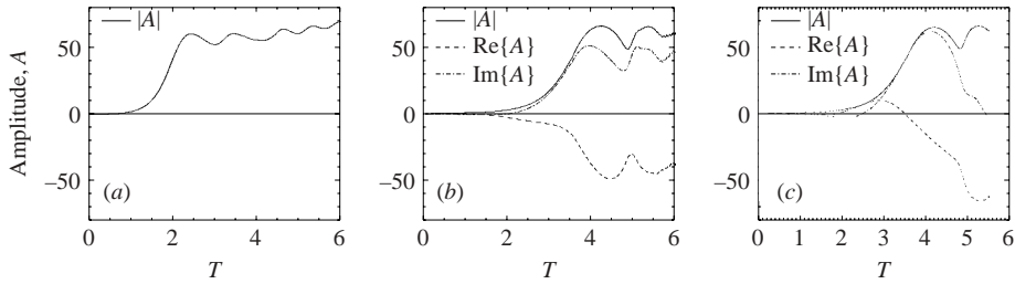
FIGURE 1. The evolution of the wave amplitude A for (a) \mathcal{D}_2=0 , (b) \mathcal{D}_2=+0.3 , (c) \mathcal{D}_2=-0.3 .
