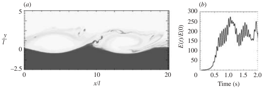
FIGURE 9. Results from direct numerical simulations with G=0.1 and r=0.1 , obtained at a (dimensional) time of \sim 1 s. (a) Density contour plot of a wind-driven gravity wave; (b) the energy of the wave as a function of time.
